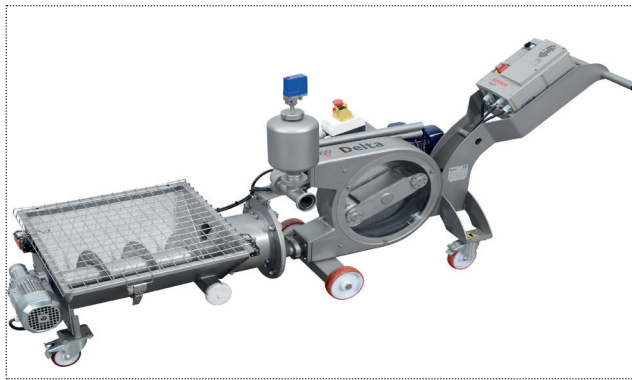
Peristaltic pump for grapes
